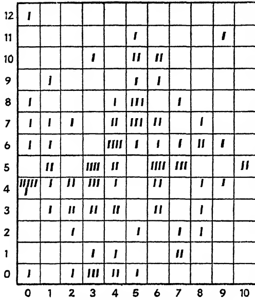
FIG. XI. Scatter diagram. Correlation of approximately +0.1.
